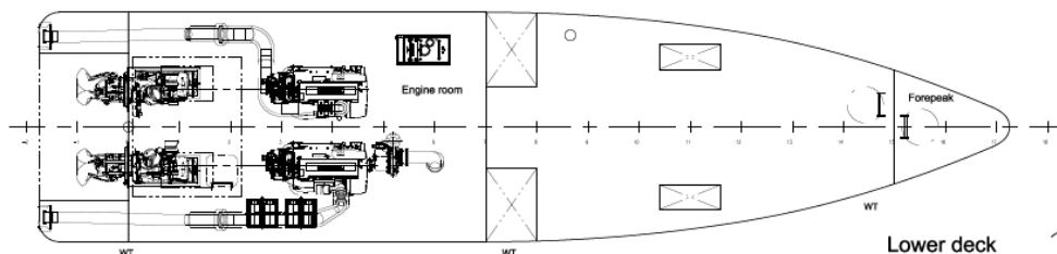
Lower deck
