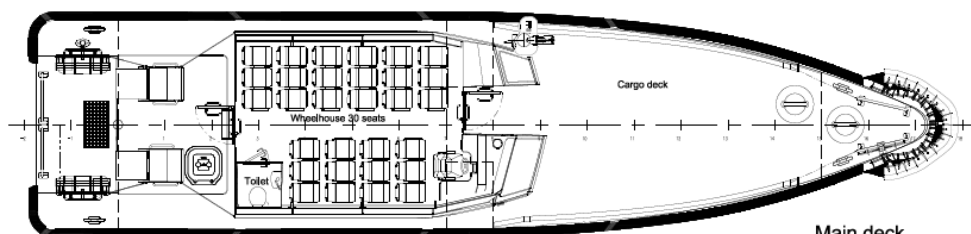
Main deck
