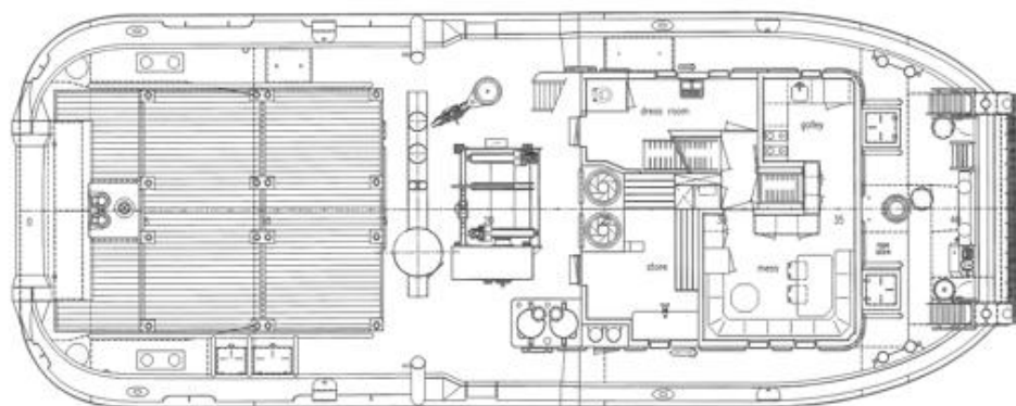
MAIN DECK
