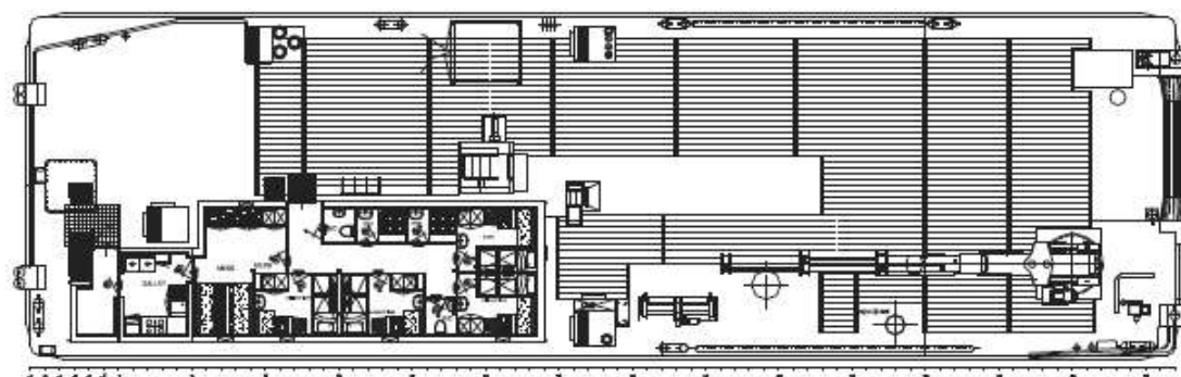
Main deck
